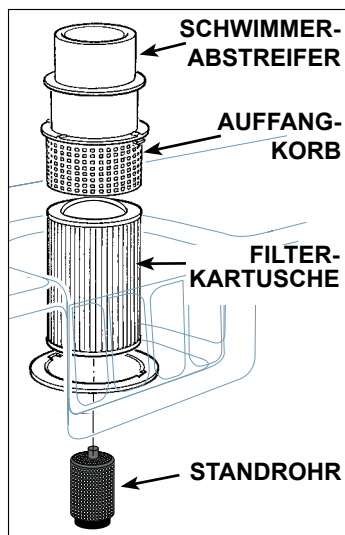
FILTERSYSTEM
