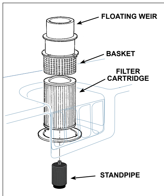
FILTER SYSTEM
