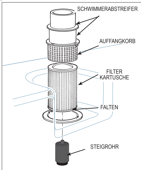
FILTERSYSTEM
